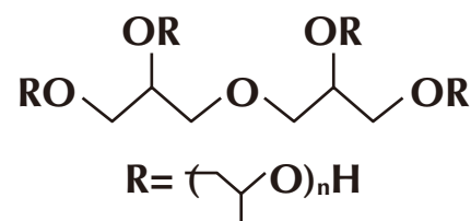
Chemical Structure
